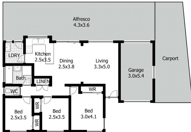
FLOOR PLAN
