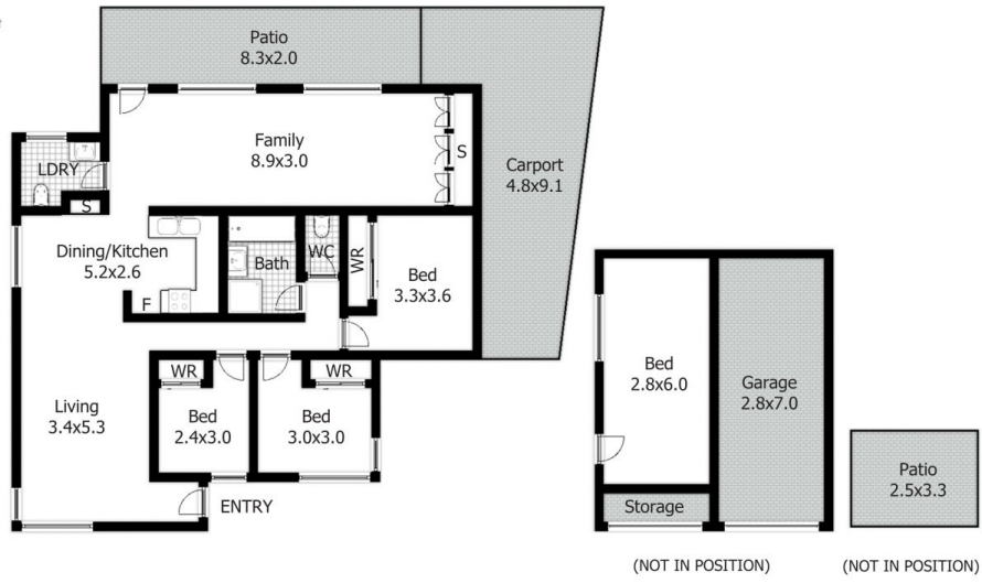
FLOOR PLAN
